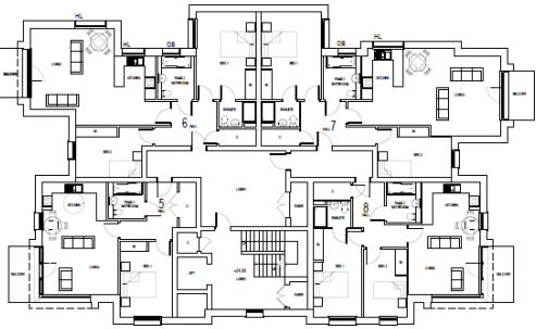
BUILDING E - First Floor
