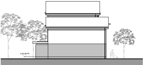
BUILDING B1 - SOUTH ELEVATION
