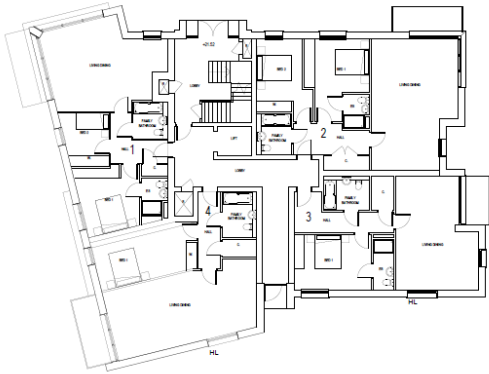
BUILDING A - GROUND FLOOR PLAN
