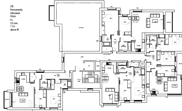
BUILDING D Third Floor
