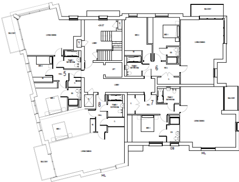
BUILDING A - FIRST FLOOR PLAN
